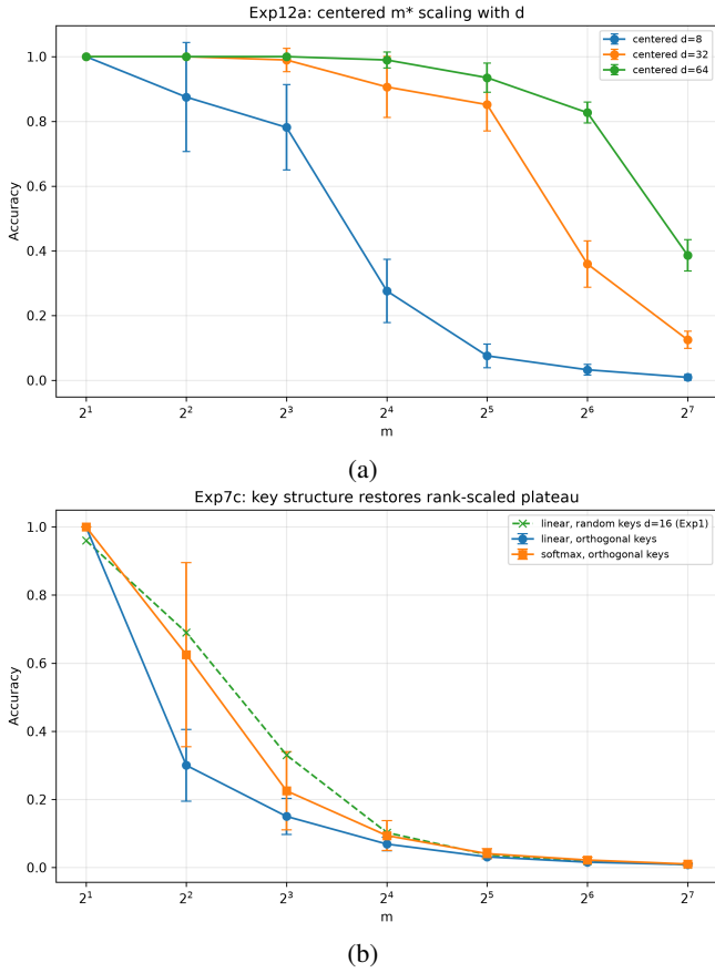
Figure 6: Measured. (a) Centered-feature recall across d = 8, 32, 64 ( n = 12 ); the first grid point at or below 0.5 moves with dimension under these centered Gaussian-key conditions. (b) Orthogonal versus random keys under elu+1 at d = 16 , with the centered-orthogonal curve for comparison.
