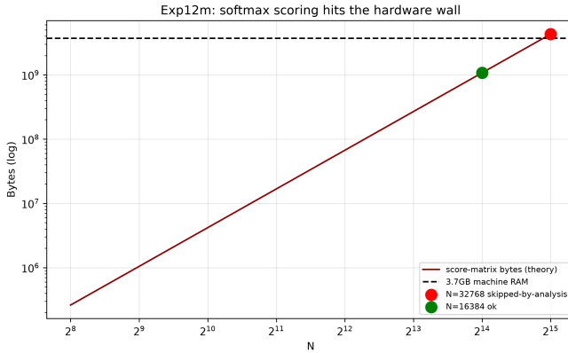
Figure 12: Measured/derived, tested implementation only. Score-matrix bytes against N for full N \times N fp32 scoring, with the 3.7 GB machine limit. The N = 16,384 case completed; N = 32,768 (4.3 GB) exceeds the limit and was not run.
