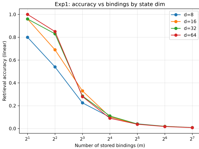
Figure 3: Measured. Retrieval accuracy versus binding count m for d = 8 – 64 under elu+1 features (seed 42, n = 25 ). The curves overlap: in this configuration the breakpoint is set by density, not by state dimension.
