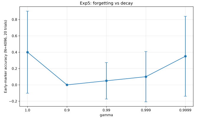
Figure 9: Measured. Early-marker accuracy at N = 4096 across retention factors \gamma \in \{1.0, 0.9, 0.99, 0.999, 0.9999\} ( n = 20 ). Error bars are sample standard deviations; the ordering across this grid is not monotone.
