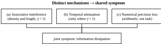
Figure 14: Conceptual schematic; no measured data. The three measured mechanisms and the single symptom they share. Grouping of length-dependent degradation under (a) follows the argument of Section VI.
