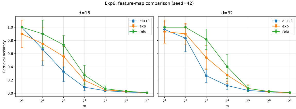
Figure 4: Measured. Feature-map comparison at d = 16 and d = 32 ( n = 15 ). The choice of \phi shifts the density curve substantially in configurations where changing d does not.
