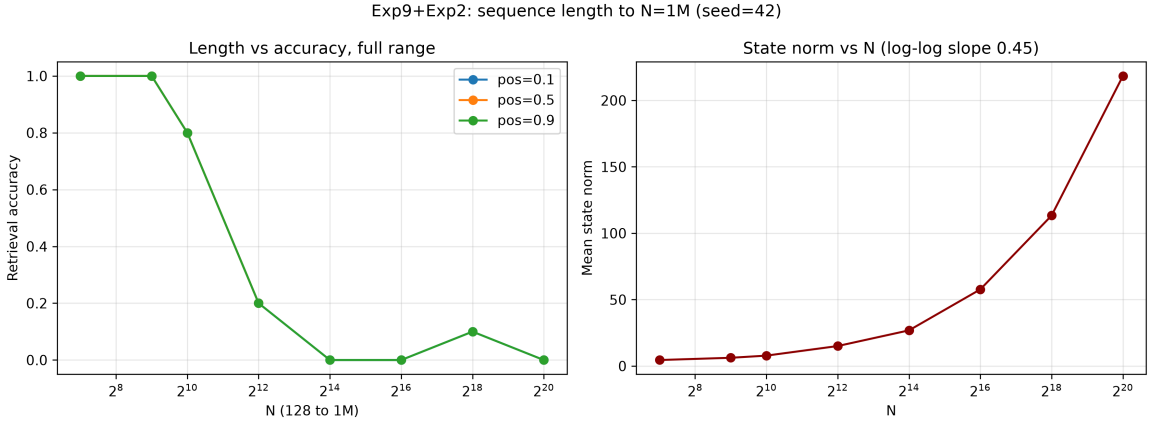
Figure 7: Measured. Left: marker recall across N for three marker positions, to N = 1\text{M} . Right: mean state norm across the same range; the combined log-log slope is 0.448. Far-end points rest on n = 2-3 .
