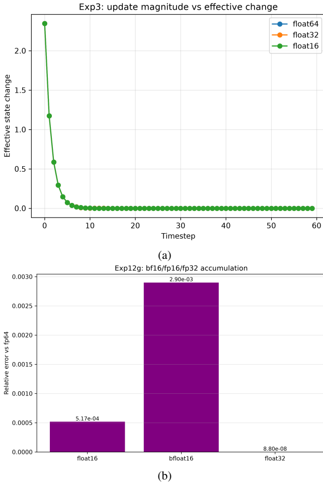
Figure 10: Measured, single-run probes. (a) Effective state change per step for shrinking updates in fp64, fp32, and fp16 over a 60-step probe at d = 8 . (b) Relative accumulation error against an fp64 reference for fp16, real bf16, and fp32 on the same probe.
