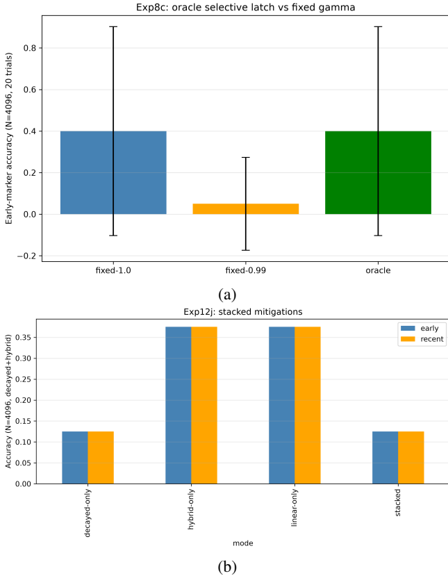
Figure 15: Measured. (a) Early-marker accuracy at N = 4096 under fixed retention and under the oracle salience latch ( n = 20 ). (b) Stacked decay plus hybrid window against each component alone, at early and recent marker positions ( N = 4096 , n = 8 ).
