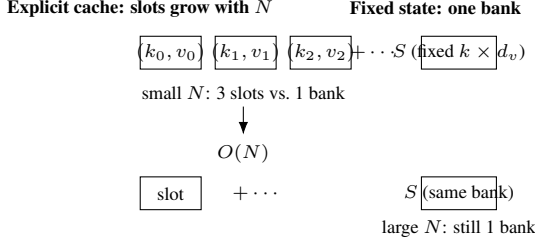
Figure 1: Conceptual schematic; no measured data. Explicit per-token storage grows with N while the fixed state remains one bank of k \times d_v numbers, which is the structural difference analyzed in Section III-C.
