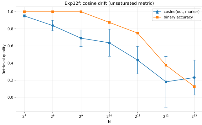
Figure 8: Measured. Cosine similarity between retrieved output and stored marker across N ( n = 8 ), alongside binary accuracy. The cosine metric resolves a gradual decline in a regime where relative error has already saturated.
