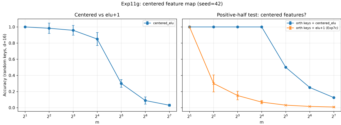
Figure 5: Measured. Left: centered-feature recall at d = 16 shows a plateau followed by a knee ( n = 15 ). Right: the positive-half comparison for orthogonal keys under centered features and under elu+1. The plateau-then-knee shape appears only with centered features; under elu+1 the decline starts at low density.
