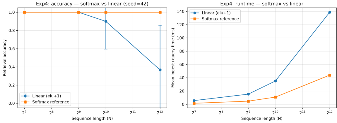
Figure 11: Measured, tested implementations only. Left: retrieval accuracy for the explicit-cache reference and the synthetic recurrence across N . Right: mean ingest-plus-query time for the same runs. Runtime reflects this single-threaded NumPy CPU build and protocol, not the architectures in general.
